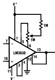
a. Input Offset Adj. for 16-Pin Package
