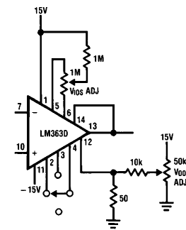
c. Input and Output Offset Adjustment for 16-Pin Package
