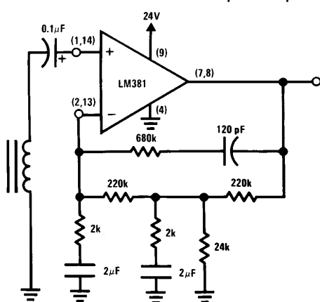
Two-Pole Fast Turn-On NAB Tape Preamp
