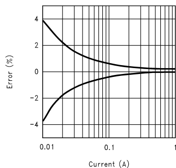
Error vs Current (LM3812-1.0 and LM3813-1.0) (Note 10)
