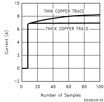
FIGURE 7. Transient Response to 7 Amp Step Current
