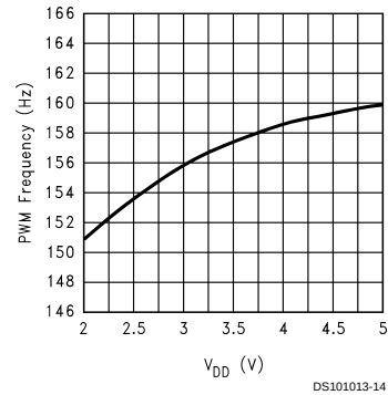
PWM Frequency vs Supply Voltage
