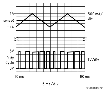
Current vs Duty Cycle
