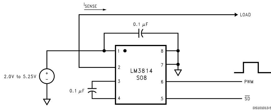
FIGURE 1. High Side Sense
