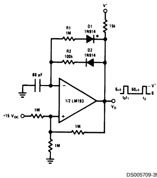
Pulse Generator
