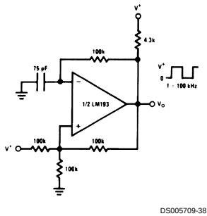
Squarewave Oscillator
