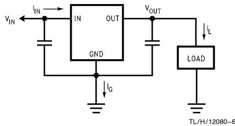
FIGURE 2. Power Dissipation Diagram
