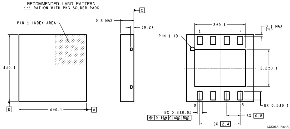
8-Lead LLP Order Part Number LM3940LD-3.3 NSC Package Number LDC08A
