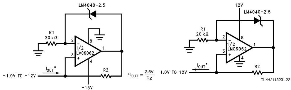
FIGURE 7. Precision 1 \mu A to 1 mA Current Sources
