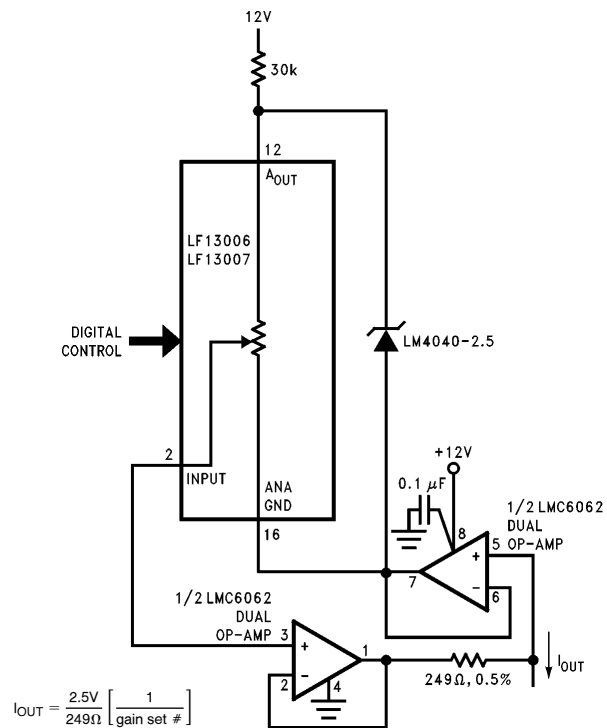
FIGURE 6. Programmable Current Source
