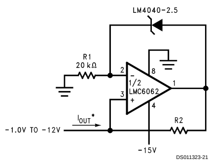
FIGURE 6. Precision 1\text{ }\mu\text{A} to 1\text{ mA} Current Sources
