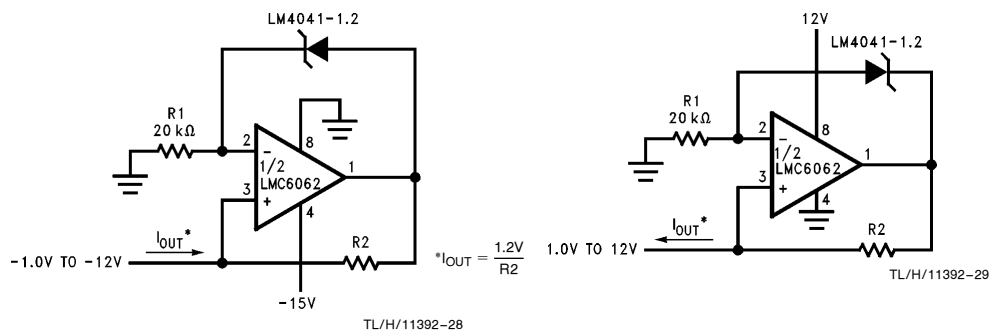
FIGURE 13. Precision 1 \mu A to 1 mA Current Sources
