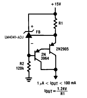
FIGURE 10. Current Source
