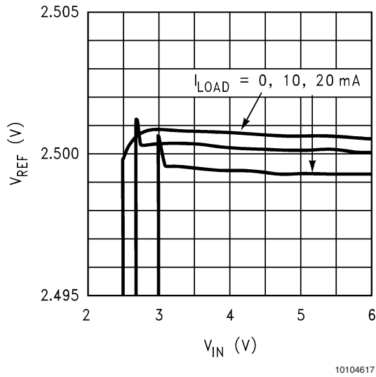
Line Regulation vs Load
