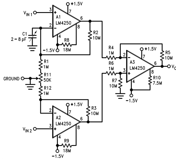
X100 Instrumentation Amplifier 10 \mu W
