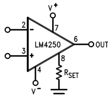
R_{SET} Connected to Ground
