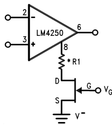
FET Current Sourcing Biasing
