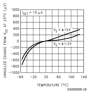
Unnull Input Offset Voltage Change vs Temperature
