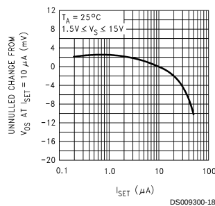
Unnull Input Offset Voltage Change vs I_{SET}
