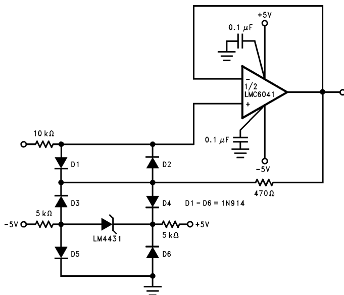
FIGURE 3. Protecting Op Amp input. The bounding voltage is ±4V with the LM4431 (LM4431's reverse breakdown voltage + 3 diode V F ).
