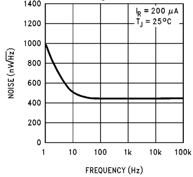
Noise Voltage
