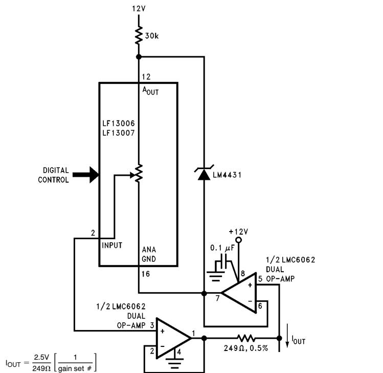
FIGURE 4. Programmable Current Source
