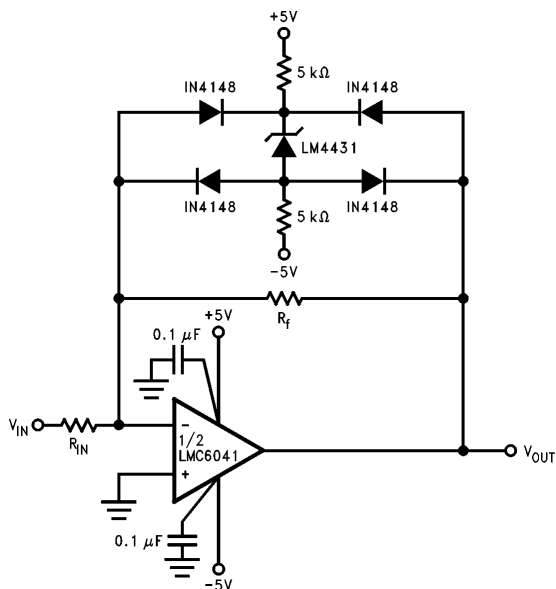
FIGURE 2. Bounded amplifier reduces saturation-induced delays and can prevent succeeding stage damage. Nominal clamping voltage is ±3.9V (LM4431's reverse breakdown voltage + 2 diode V F ).
