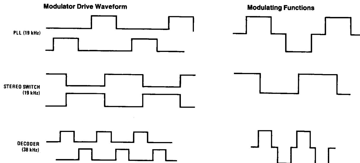
FIGURE 3. Digital Waveforms
