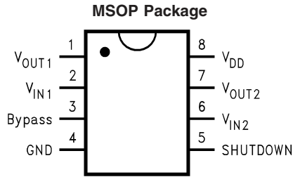
20008902 Top View Order Number LM4810MM See NS Package Number MUA08A
