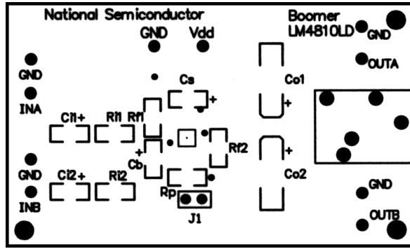
FIGURE 6. Recommended LD PC Board Layout Component-Side Silkreen
