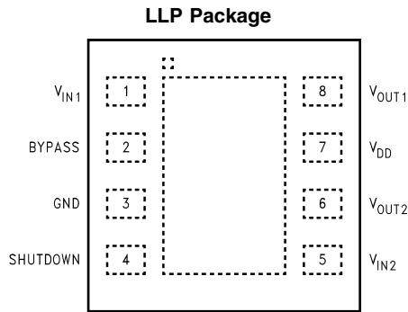
20008986 Top View Order Number LM4810LD See NS Package Number LDA08B
