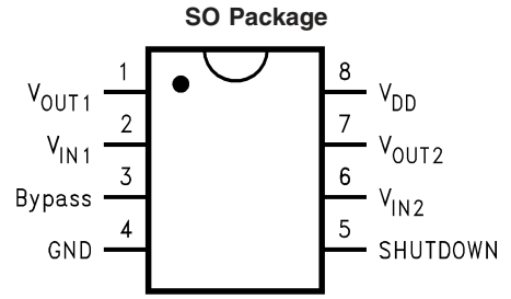
20008902 Top View Order Number LM4810MA See NS Package Number M08A
