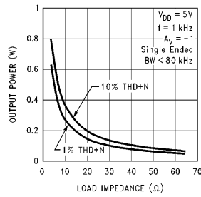
Output Power vs Load Impedance
