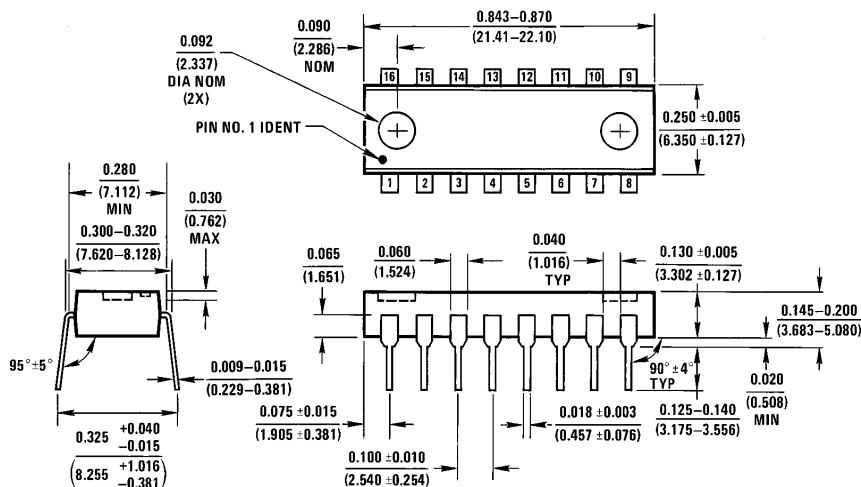
16-Lead (0.300" Wide) Molded Dual-In-Line Package Order Number LM4863 NS Package Number N16A
