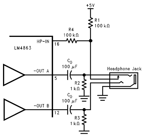
FIGURE 2. Headphone Input Circuit
