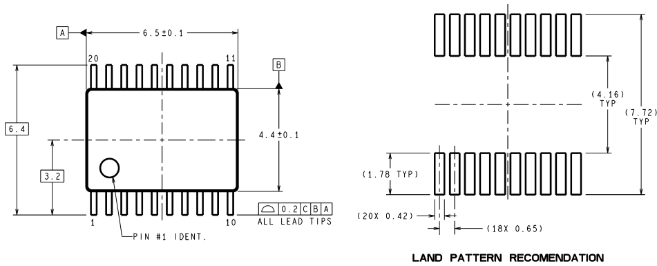
LAND PATTERN RECOMENDATION
