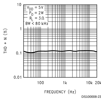
LM4871LD THD+N vs Frequency
