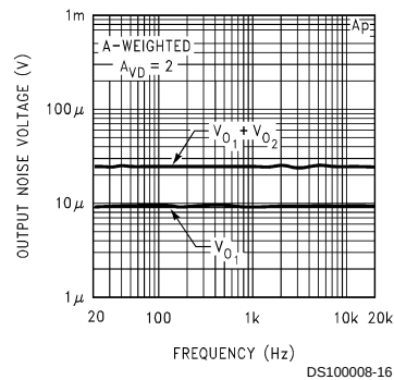
Noise Floor
