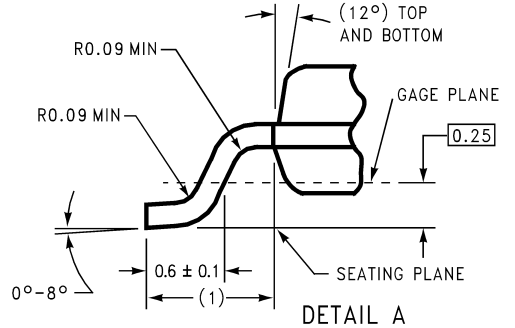
DETAIL A TYPICAL, SCALE: 40X
