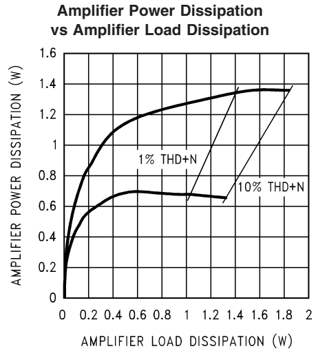
V_{DD} = 5\text{V} , f_{IN} = 1\text{kHz} , at (from top to bottom at 1W): R_L = 4\Omega , R_L = 8\Omega , single channel driven and loaded
