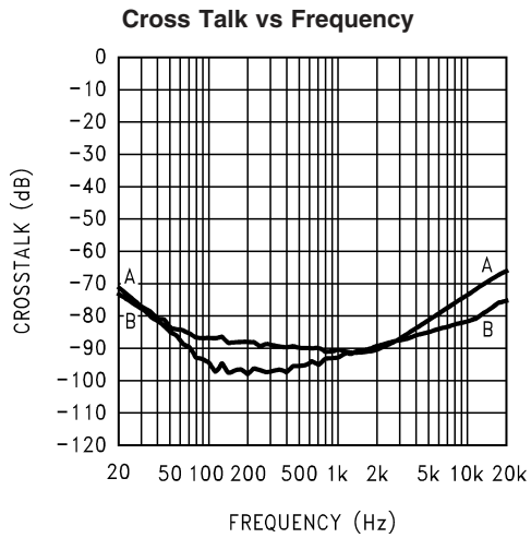
200469D1 V_{DD} = 5V, R_L = 8\Omega, A_V = 15.6dB, A = Left channel driven, right channel measured; B = Right channel driven, left channel measured
