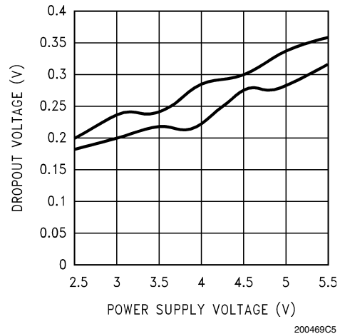
Dropout Voltage vs Power Supply Voltage
