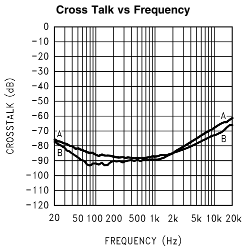
200469D2 V_{DD} = 5V, R_L = 8\Omega, A_V = 21.6dB, A = Left channel driven, right channel measured; B = Right channel driven, left channel measured
