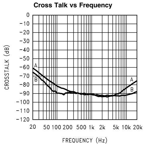
V_{DD} = 5\text{V} , R_L = 8\Omega , A_V = 6\text{dB} , A = Left channel driven, right channel measured; B = Right channel driven, left channel measured
