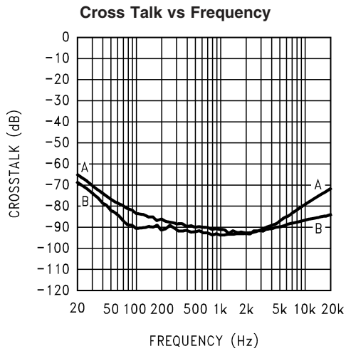
200469D0 V_{DD} = 5V, R_L = 8\Omega, A_V = 10dB, A = Left channel driven, right channel measured; B = Right channel driven, left channel measured
