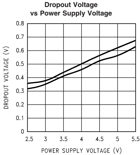
R_L = 4\Omega , f_{IN} = 1\text{kHz} , both channels driven and loaded at (from top to bottom at 4V): positive signal swing, negative signal swing
