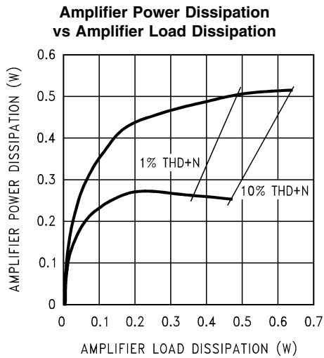
V_{DD} = 3\text{V} , f_{IN} = 1\text{kHz} , at (from top to bottom at 0.3W): R_L = 4\Omega , R_L = 8\Omega , single channel driven and loaded
