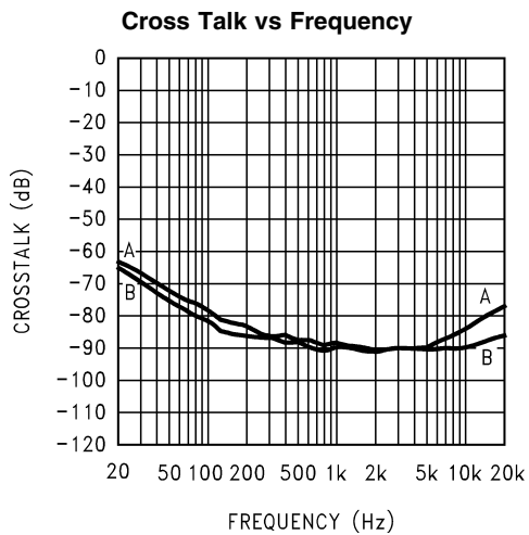
200469D3 V_{DD} = 3V, R_L = 8\Omega, A_V = 6dB, A = Left channel driven, right channel measured; B = Right channel driven, left channel measured
