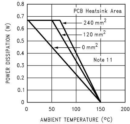
Power Derating - 8 Bump \mu SMD P_{DMAX} = 670mW for 5V, 8Ω
