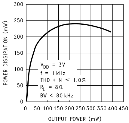
Power Dissipation vs Output Power V_{DD} = 3.0V
