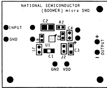
Silk Screen
