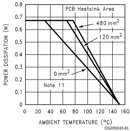
Power Derating - 9 Bump \mu SMD P_{DMAX} = 670mW for 5V, 8Ω
