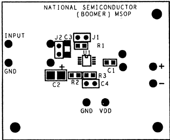
Silk Screen
