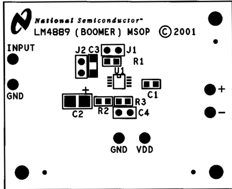
Silk Screen
