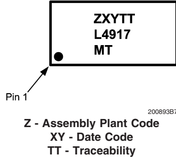
TSSOP Marking
