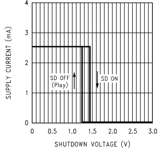
Shutdown Hysteresis Voltage V_{DD} = 5V, SD Mode = V_{DD}
