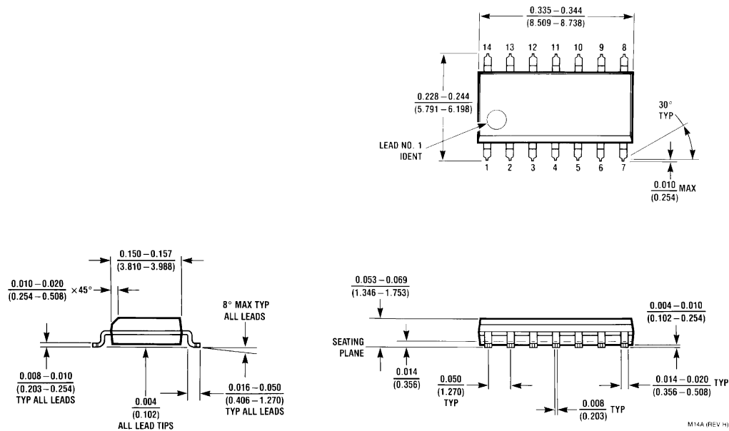
14-Lead (0.150") Molded Small Outline Package, JEDEC Order Number LM6154ACM or LM6154BCM NSC Package Number M14A
