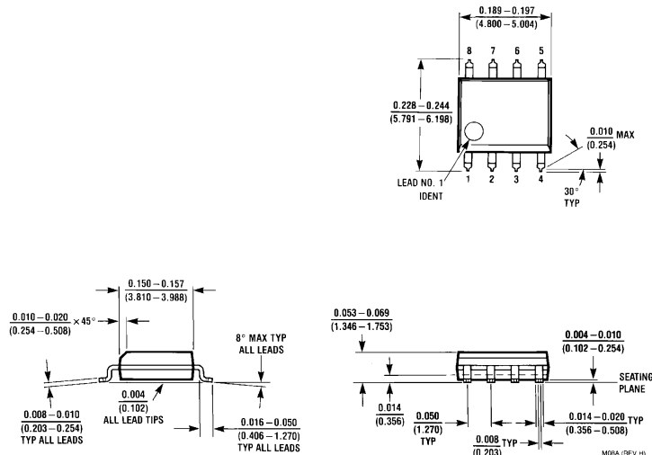
8-Lead (0.150") Molded Small Outline Package, JEDEC Ordering Number LM6152ACM or LM7162BCM NSC Package Number M08A
