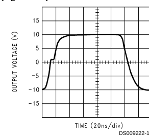
Large Signal Response ( R_L = 50\Omega )
