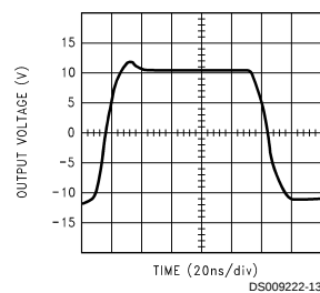
Large Signal Response ( R_L = 1\text{ k}\Omega )
