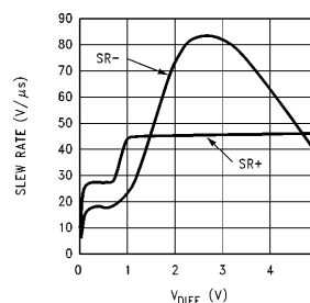
FIGURE 2. Slew Rate vs V_{DIFF}
