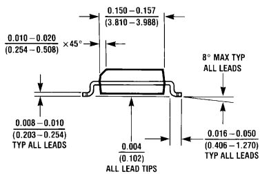
14-Lead (0.150" Wide) Molded Small Outline Package, JEDEC Order Number LM6154ACM or LM6154BCM NS Package Number M14A
