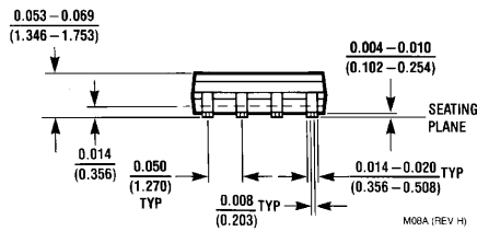
8-Lead (0.150" Wide) Molded Small Outline Package, JEDEC Order Number LM6152ACM or LM6152BCM NS Package Number M08A
