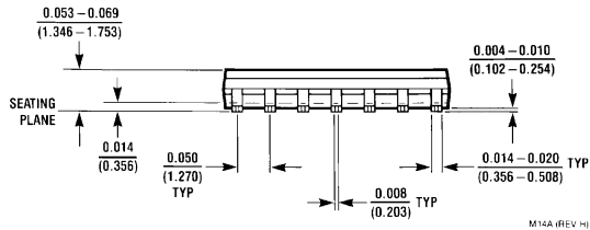
14-Lead (0.150" Wide) Molded Small Outline Package, JEDEC Order Number LM6154ACM or LM6154BCM NS Package Number M14A
