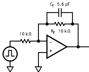
FIGURE 1. Typical Inverting Gain Circuit A_V = -1
