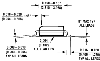
8-Lead (0.150" Wide) Molded Small Outline Package, JEDEC Order Number LM6152ACM or LM6152BCM NS Package Number M08A
