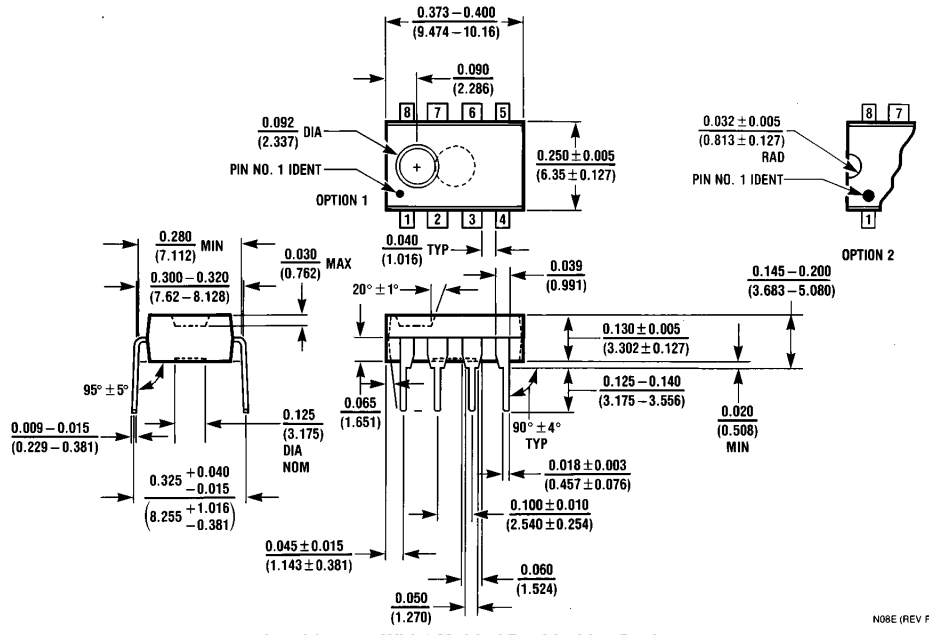
8-Lead (0.300" Wide) Molded Dual-In-Line Package Order Number LM6152ACN or LM6152BCN NS Package Number N08E
