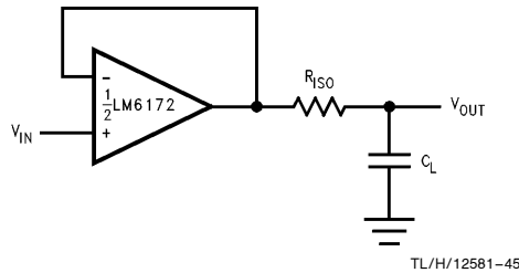
FIGURE 1. Isolation Resistor Used to Drive Capacitive Load
