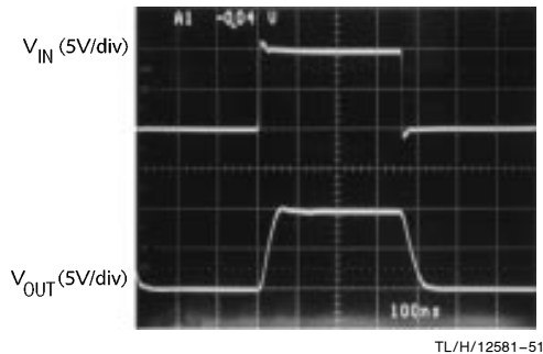
FIGURE 2. The LM6172 Driving a 510 pF Load with a 30 \Omega Isolation Resistor
