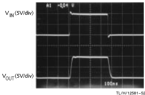
FIGURE 3. The LM6172 Driving a 220 pF Load with a 50 \Omega Isolation Resistor
