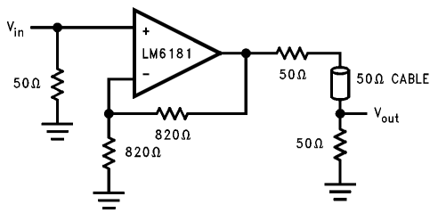
Cable Driver
