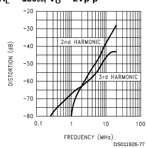
Distortion vs Frequency V_S = \pm 5V , A_V = +2 , R_L = 150\Omega , V_O = 2Vp-p
