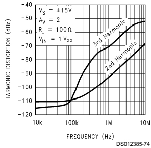
Harmonic Distortion vs Frequency
