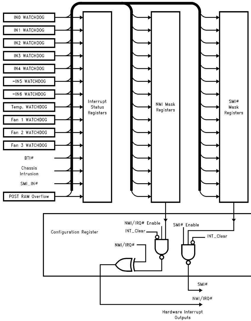
FIGURE 12. Interrupt Structure
