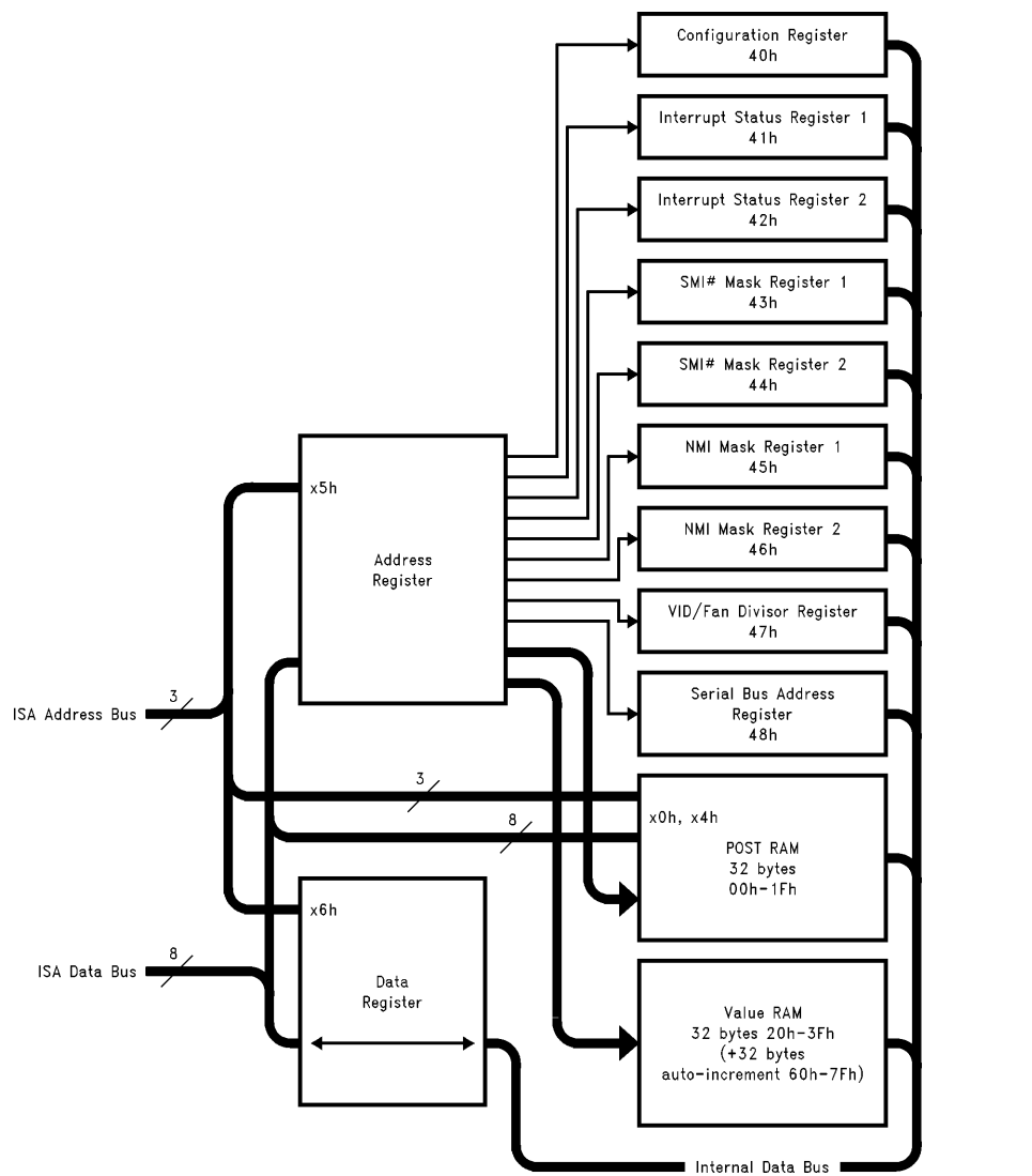
FIGURE 6. LM78 Register Structure
