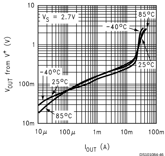
Output Voltage vs. Output Sourcing Current
