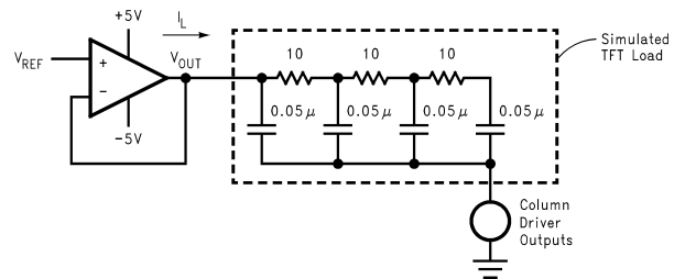
FIGURE 8. V_{COM} driver application schematic
