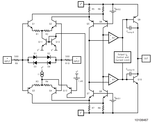
FIGURE 1. Simplified schematic Diagram
