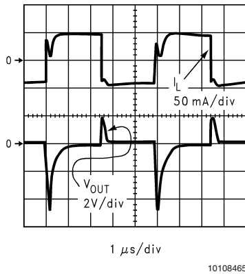
FIGURE 9. V_{COM} driver performance scope photo
