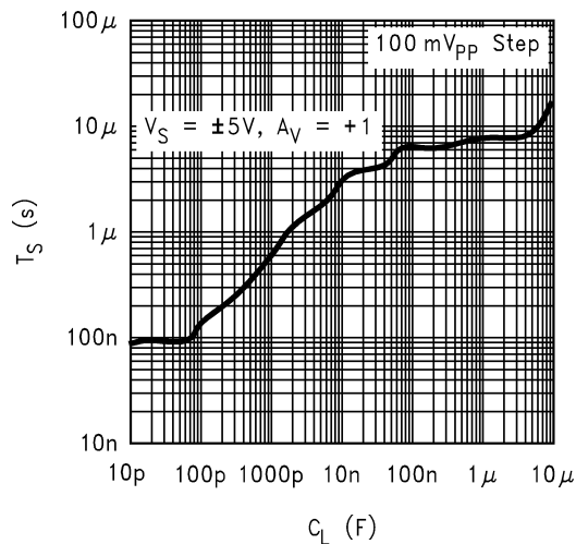
\pm 5\% Settling Time vs. Cap Load
