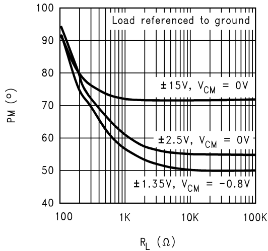
Phase Margin vs. Load
