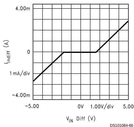
FIGURE 2. Input Stage Current vs Differential Input Voltage
