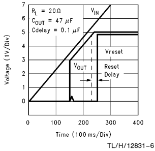
Turn ON Characteristics
