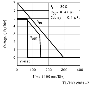
Turn OFF Characteristics
