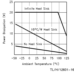
Maximum Power Dissipation (TO-220 Package)
