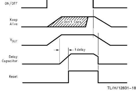
Simple ON/OFF control (Keep-Alive input must be high to turn OFF output)
