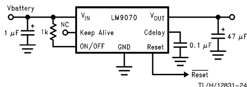
FIGURE 2. Control Logic Not Used
