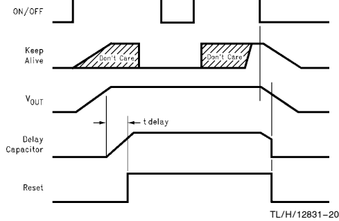
Switch ON with ON/OFF input; Keep output biased with Keep-Alive; Hold output ON with ON/OFF; Turn OFF with ON/OFF input. (Temporary Keep-Alive Mode)
