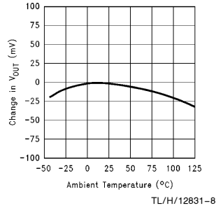
Normalized Output Voltage vs Temperature
