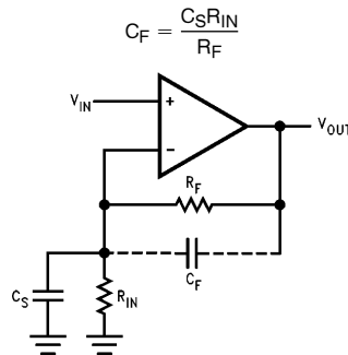
FIGURE 2. General Operational Amplifier Circuit
