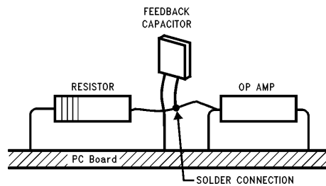
FIGURE 6. Air Wiring
