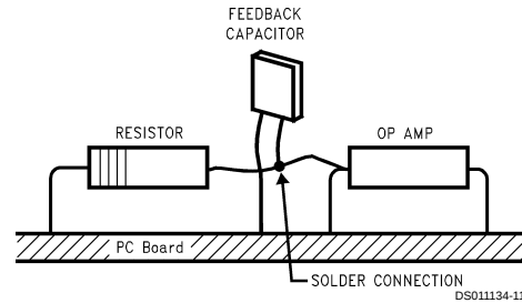
FIGURE 10. Air Wiring
