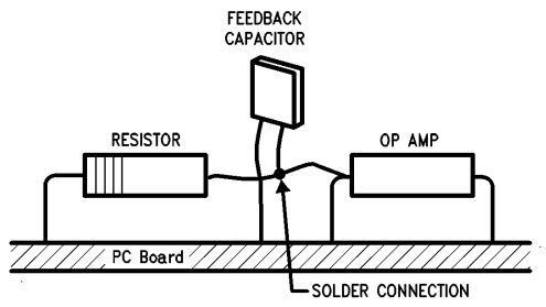
TL/H/11137-11 (Input pins are lifted out of PC board and soldered directly to components. All other pins connected to PC board.)
