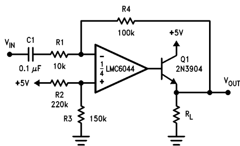
FIGURE 11. AC Coupled Power Amplifier
