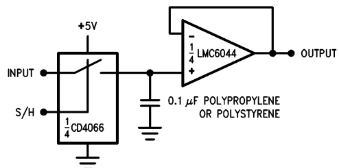
FIGURE 8. Low-Leakage Sample-and-Hold
