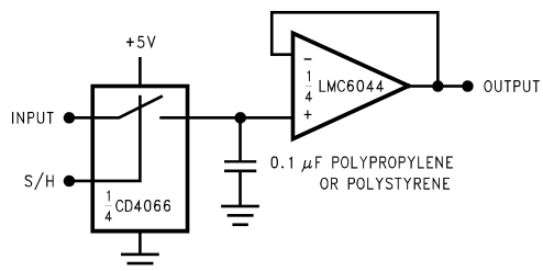
FIGURE 9. Low-Leakage Sample-and-Hold
