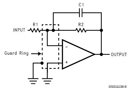
Inverting Amplifier
