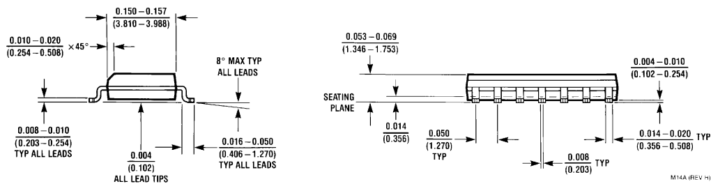
14-Pin Small Outline Package Order Number LMC6064AIM or LMC6064IM NS Package Number M14A
