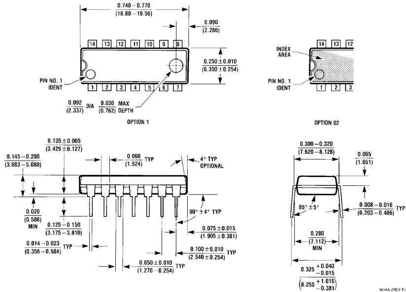
14-Pin Molded Dual-In-Line Package Order Number LMC6064AMN, LMC6064AIN or LMC6064IN NS Package Number N14A
