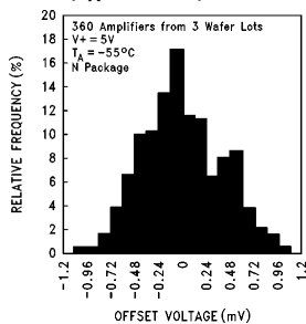
Distribution of LMC6081 Input Offset Voltage ( T_A = -55^\circ C )
