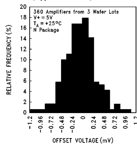
Distribution of LMC6081 Input Offset Voltage ( T_A = +25^\circ C )
