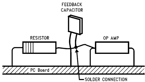
FIGURE 5. Air Wiring
