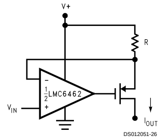
FIGURE 20. Precision Current Source
