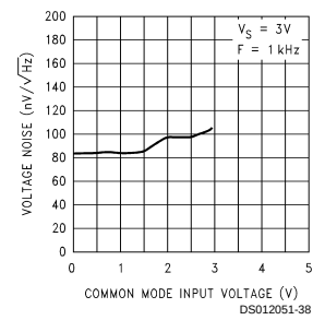
Input Voltage Noise vs Input Voltage
