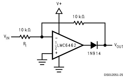
FIGURE 19. Full-Wave Rectifier with Input Current Protection ( R_1 )
