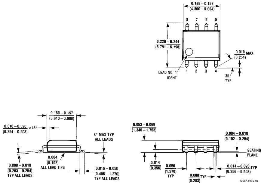
8-Pin Small Outline Package Order Number LMC6462AIM or LMC6462BIM NS Package Number M08A
