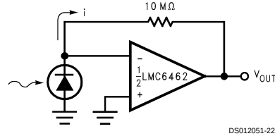
FIGURE 16. Photo Detector Circuit
