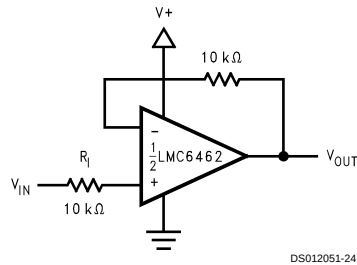
FIGURE 18. Half-Wave Rectifier with Input Current Protection ( R_1 )
