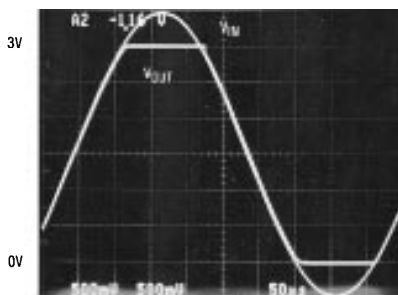
FIGURE 1. An Input Voltage Signal Exceeds the LMC6484 Power Supply Voltages with No Output Phase Inversion
