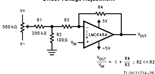
FIGURE 13. Non-Inverting Configuration Offset Voltage Adjustment
