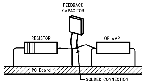
FIGURE 11. Air Wiring
