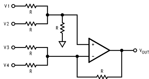
FIGURE 9. Adder/Subtractor Circuit
