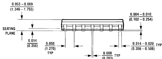
14-Pin Small Outline Package Order Package Number LMC6574AIM or LMC6574BIM NS Package Number M14A
