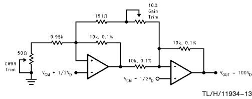
FIGURE 6. Low-Power Two-Op-Amp Instrumentation Amplifier
