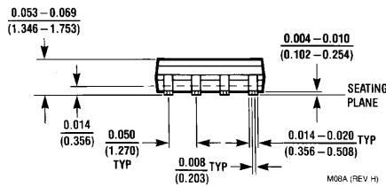
8-Pin Small Outline Package Order Package Number LMC6572AIM or LMC6572BIM NS Package Number M08A
