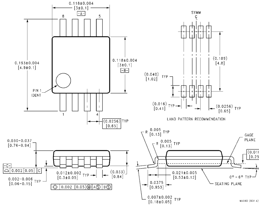
8-Lead Mini-Small Outline Molded Package, JEDEC Order Number LMC6572BIMM or LMC6572BIMMX NS Package Number MA08D
