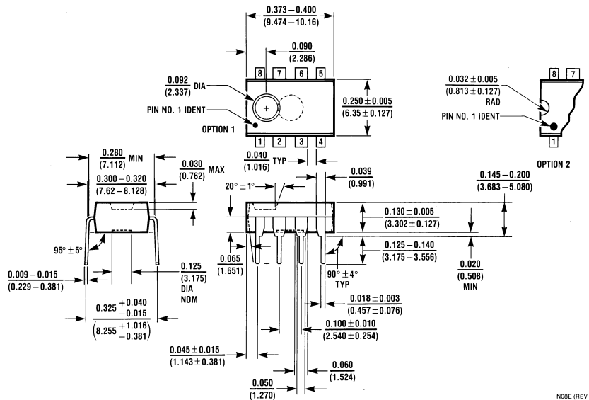
8-Pin Molded Dual-In-Line Package Order Number LMC6572AIN or LMC6572BIN NS Package Number NO8E
