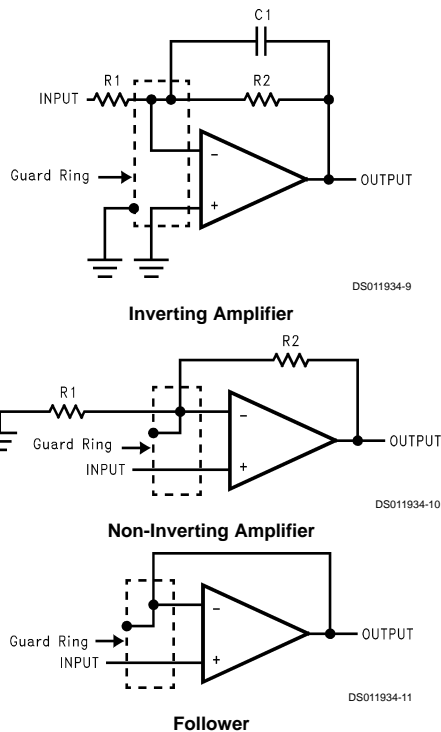
FIGURE 4. Typical Connections of Guard Rings
